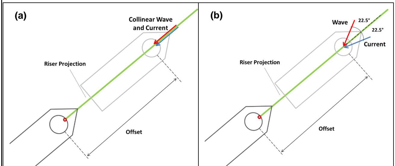
Figure 4 - Environmental conditions for SPM FPU's: (a) Head seas (b) Quartering seas
